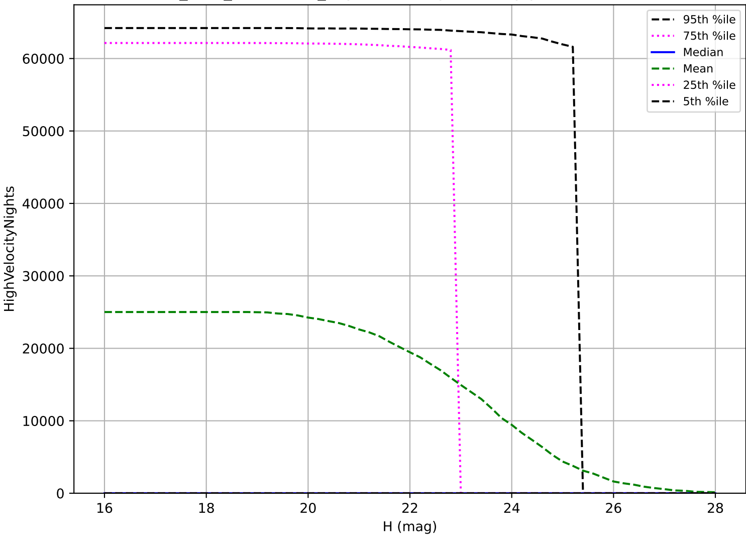
start_date_do360v3.4_10yrs: PHA High velocity pair detection loss
