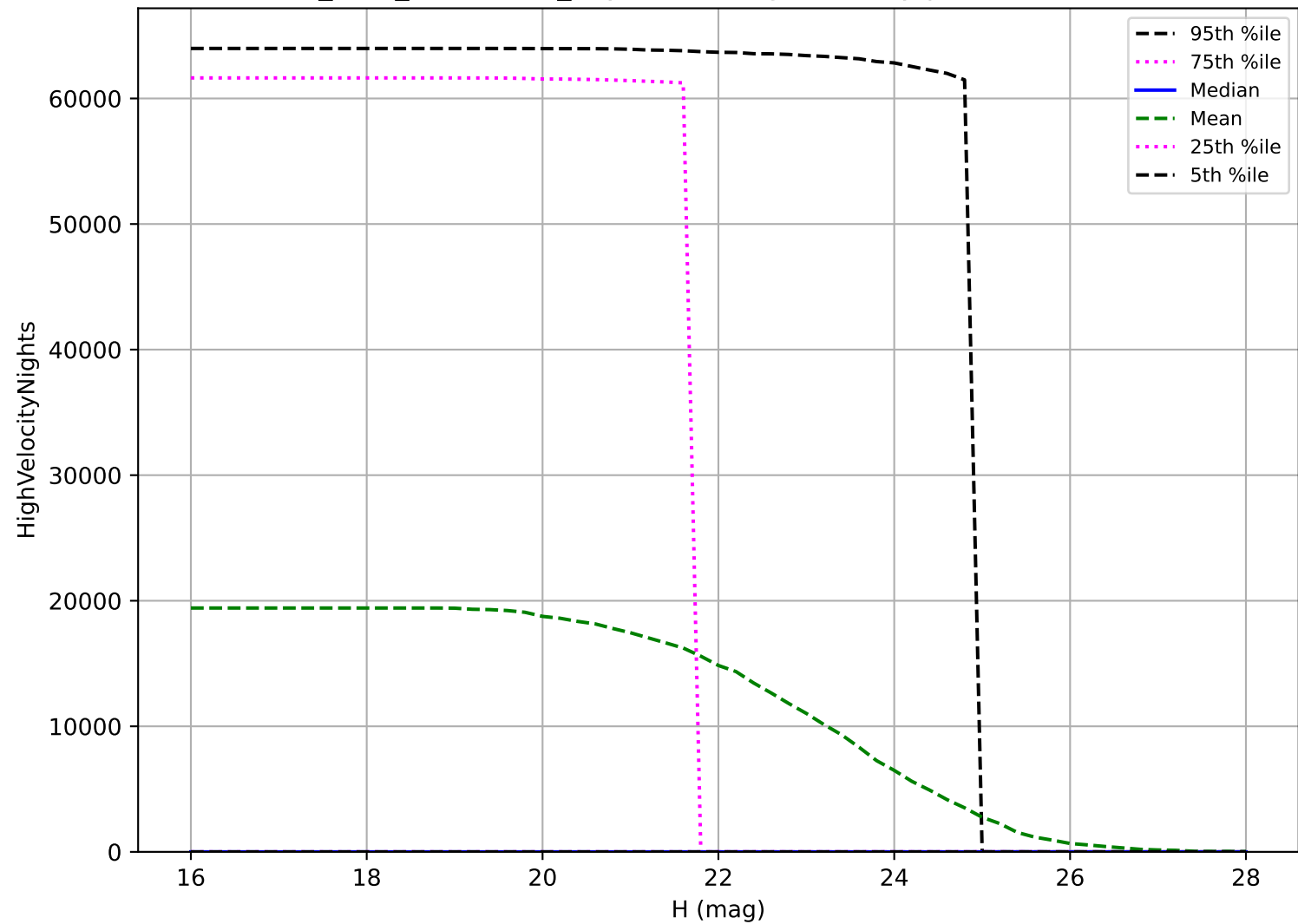
start_date_do360v3.4_10yrs: NEO High velocity pair detection loss
