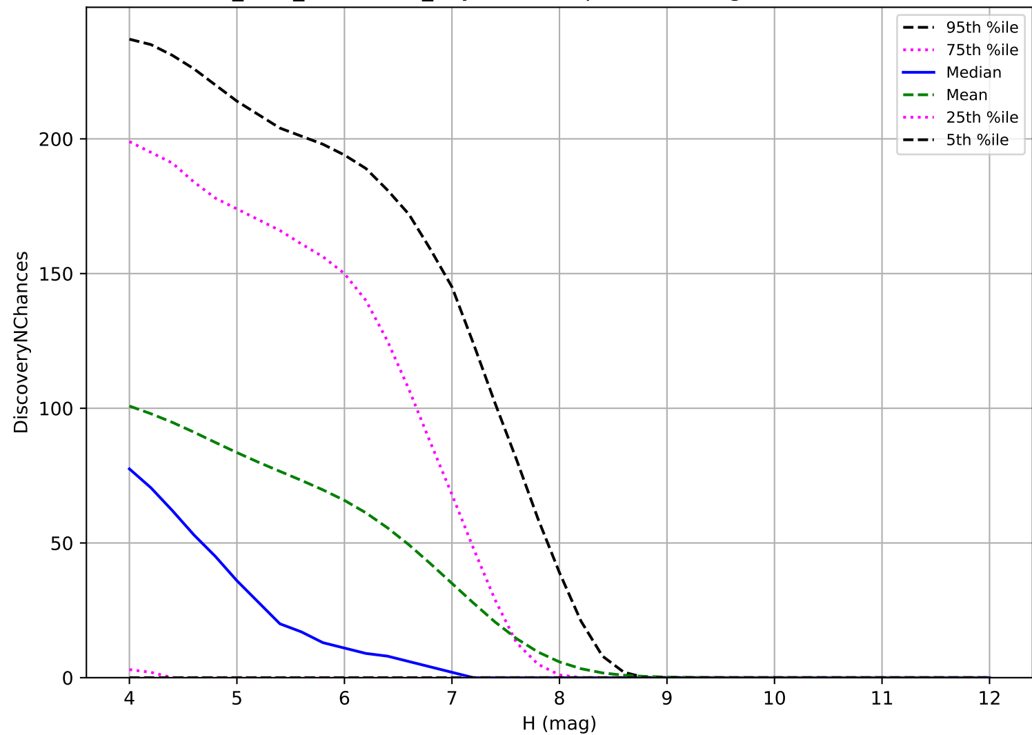
start_date_do360v3.4_10yrs: TNO 3 pairs in 15 nights detection loss
