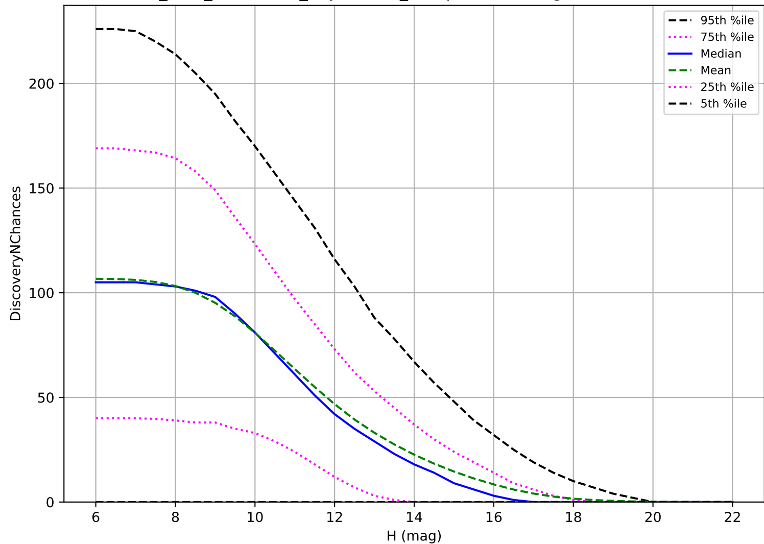
start_date_do360v3.4_10yrs: OCC_r5 3 pairs in 15 nights detection loss
