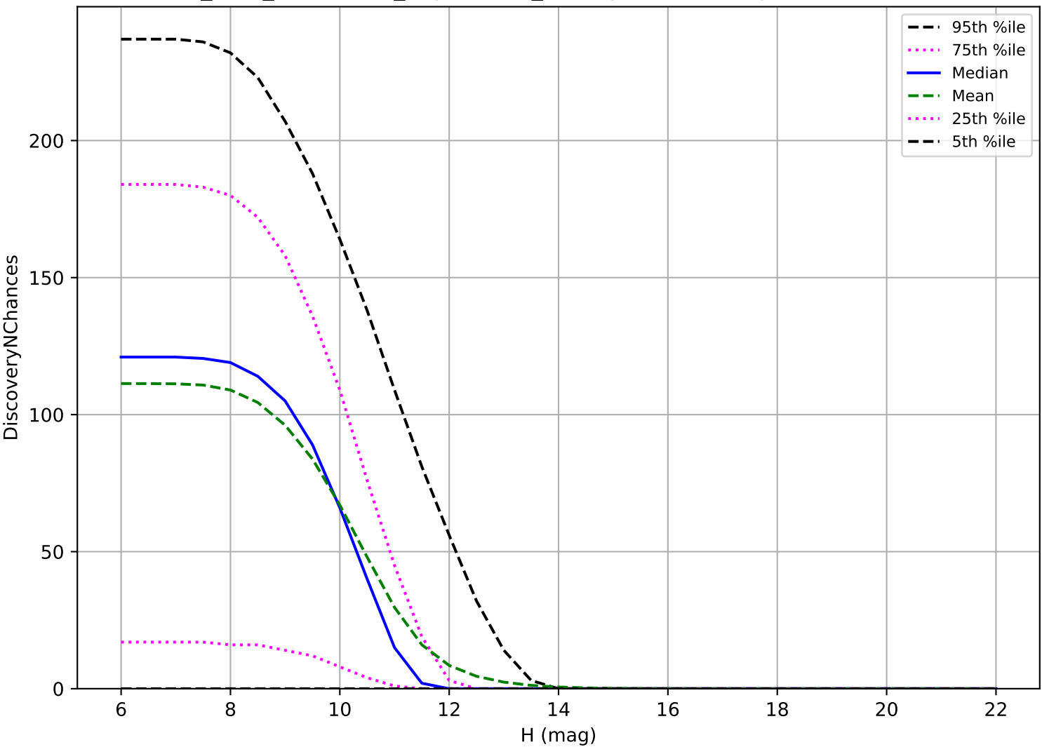
start_date_do360v3.4_10yrs: OCC_r20 3 pairs in 15 nights detection loss
