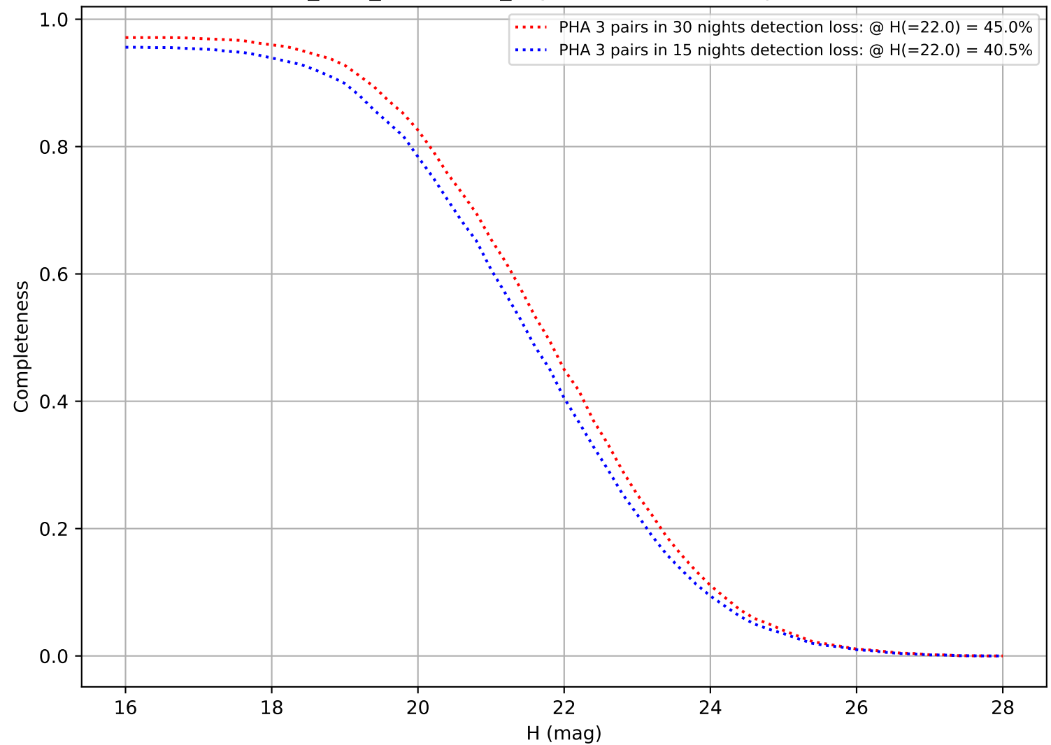
start_date_do360v3.4_10yrs: DifferentialCompleteness
