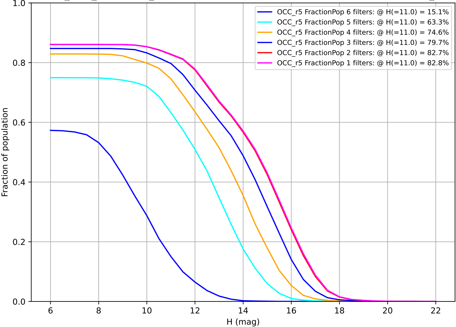
start_date_do360v3.4_10yrs: Fraction of population with colors in X filters OCC_r5
