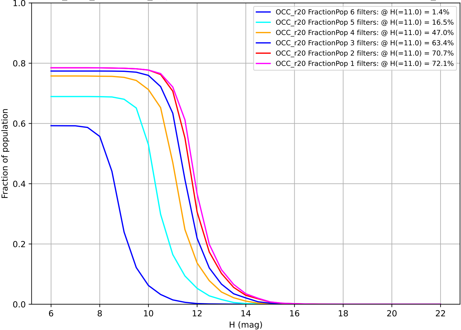
start_date_do360v3.4_10yrs: Fraction of population with colors in X filters OCC_r20
