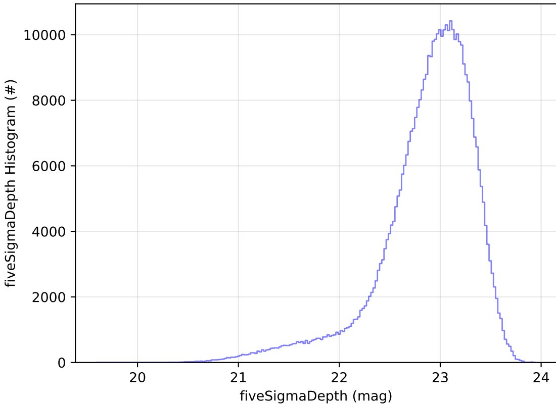
start_date_do360v3.4_10yrs z: fiveSigmaDepth Histogram
