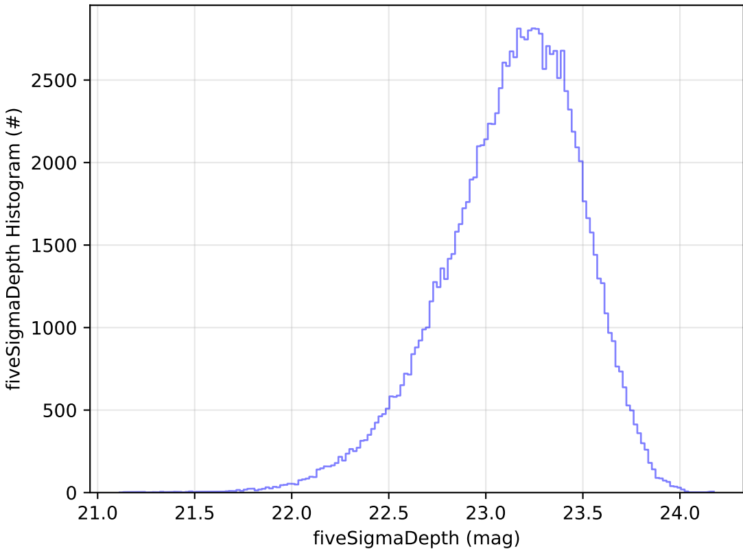
start_date_do360v3.4_10yrs u: fiveSigmaDepth Histogram
