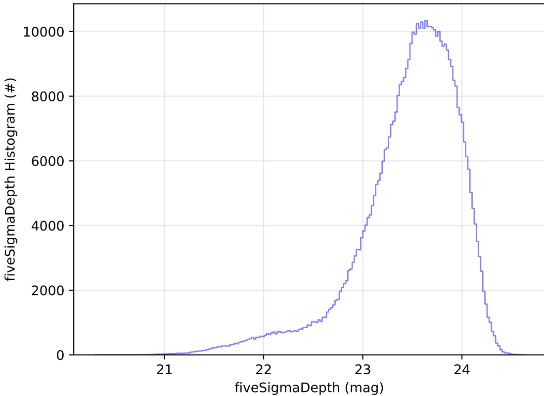
start_date_do360v3.4_10yrs i: fiveSigmaDepth Histogram
