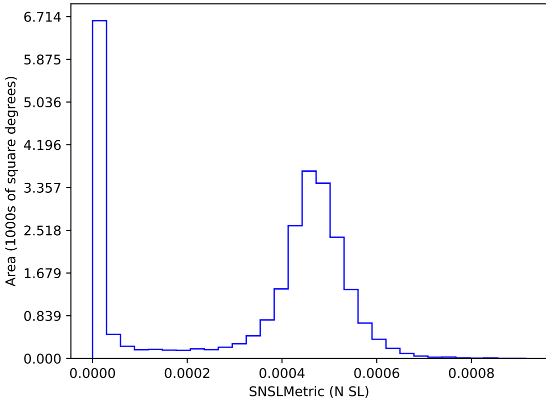
start_date_do360v3.4_10yrs : SNSLMetric
