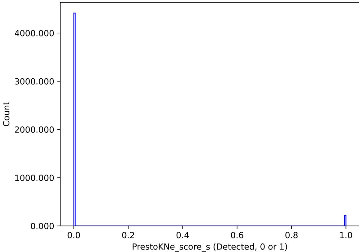
start_date_do360v3.4_10yrs : PrestoKNe_score_s
