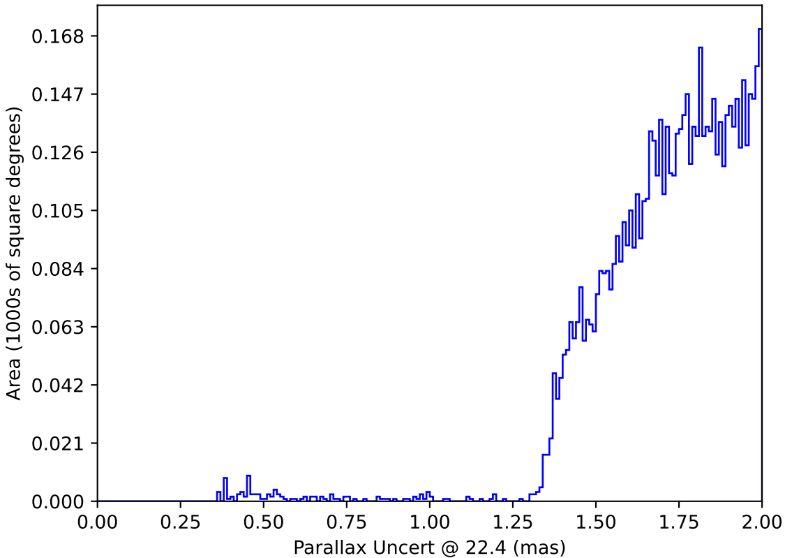
start_date_do360v3.4_10yrs : Parallax Uncert @ 22.4
