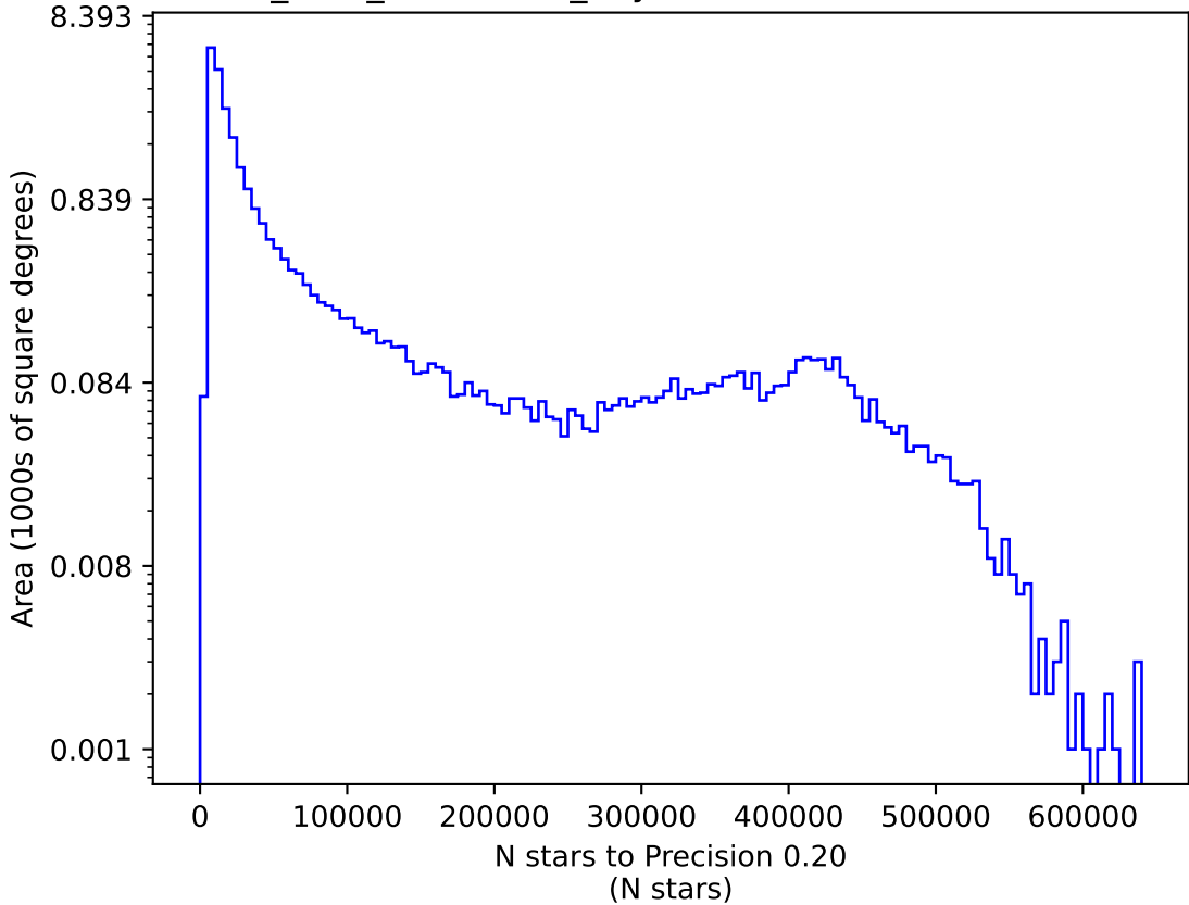
start_date_do360v3.4_10yrs i: N stars to Precision 0.20
