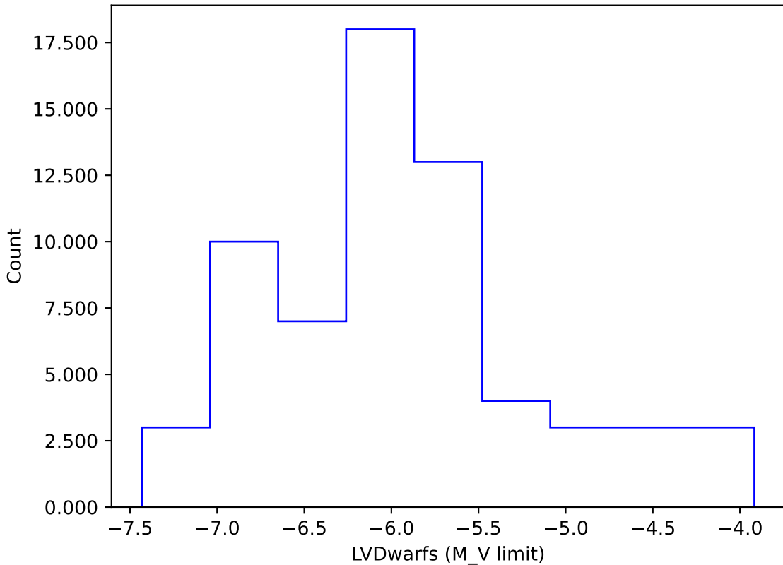
start_date_do360v3.4_10yrs gi: LVDwarfs
