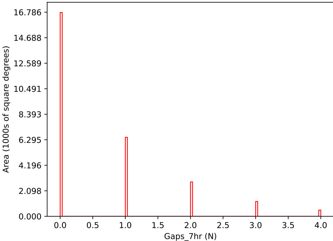
start_date_do360v3.4_10yrs i band: Gaps_7hr
