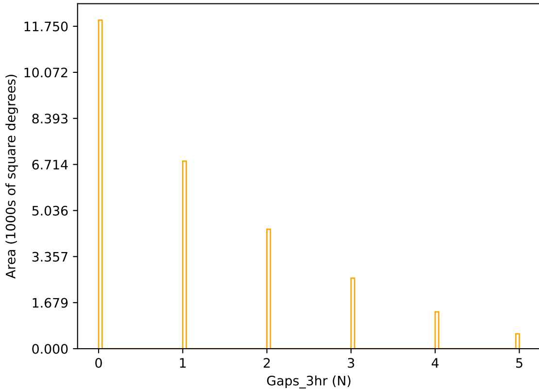
start_date_do360v3.4_10yrs r band: Gaps_3hr
