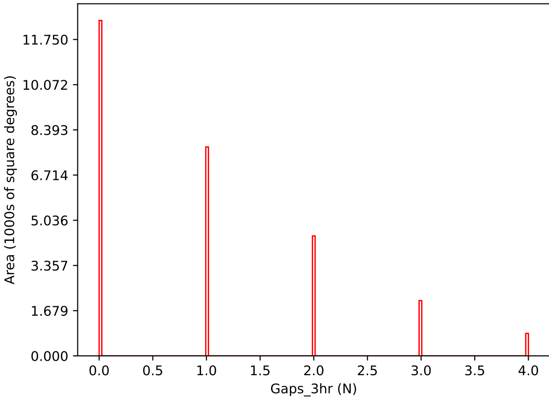
start_date_do360v3.4_10yrs i band: Gaps_3hr
