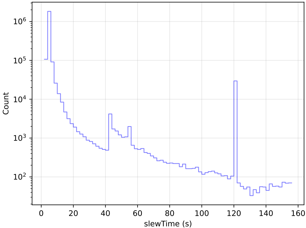
start_date_do360v3.4_10yrs All visits: Slew Time Histogram
