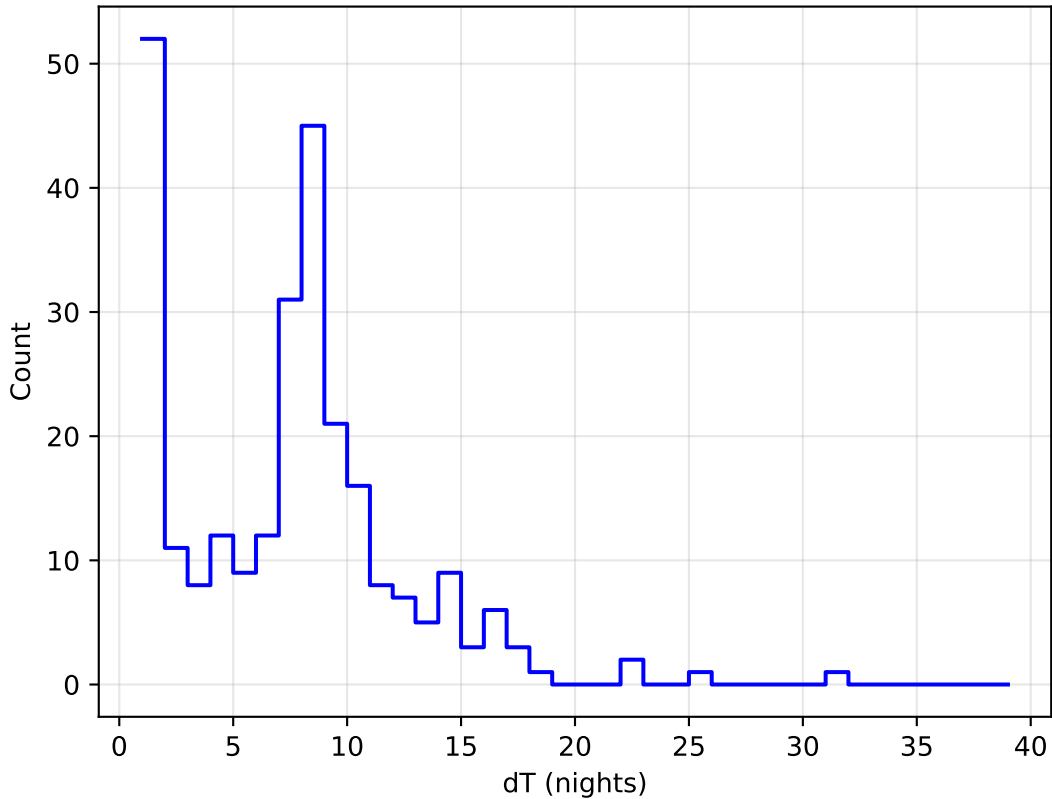
start_date_do360v3.4_10yrs all bands: DD:XMM_LSS Delta Nights Histogram
