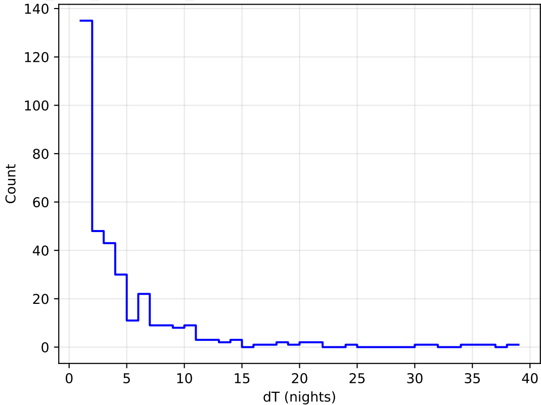
start_date_do360v3.4_10yrs all bands: DD:WFD Delta Nights Histogram
