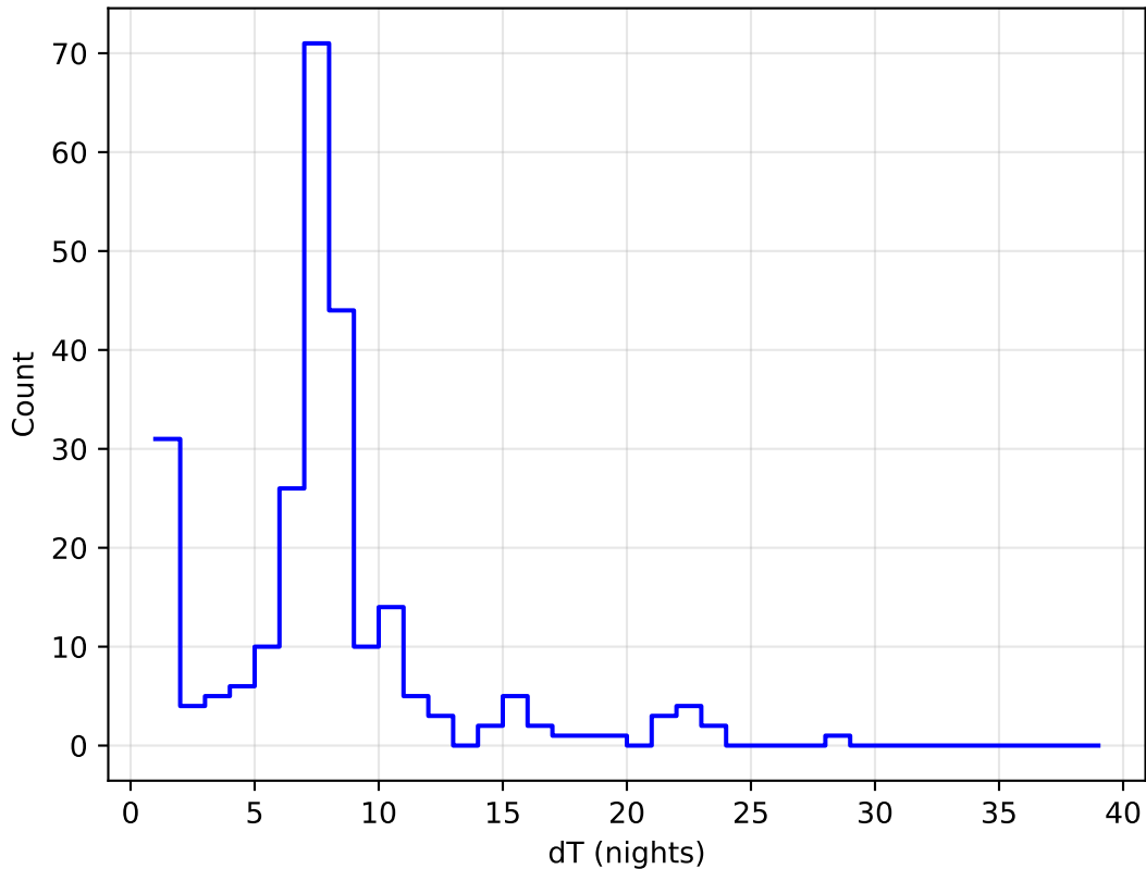
start_date_do360v3.4_10yrs all bands: DD:EDFS Delta Nights Histogram
