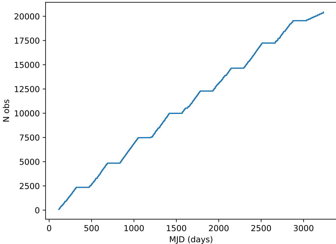
start_date_do360v3.4_10yrs all bands: DD:EDFS Cumulative NVisits
