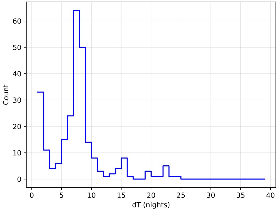
start_date_do360v3.4_10yrs all bands: DD:ECDFS Delta Nights Histogram
