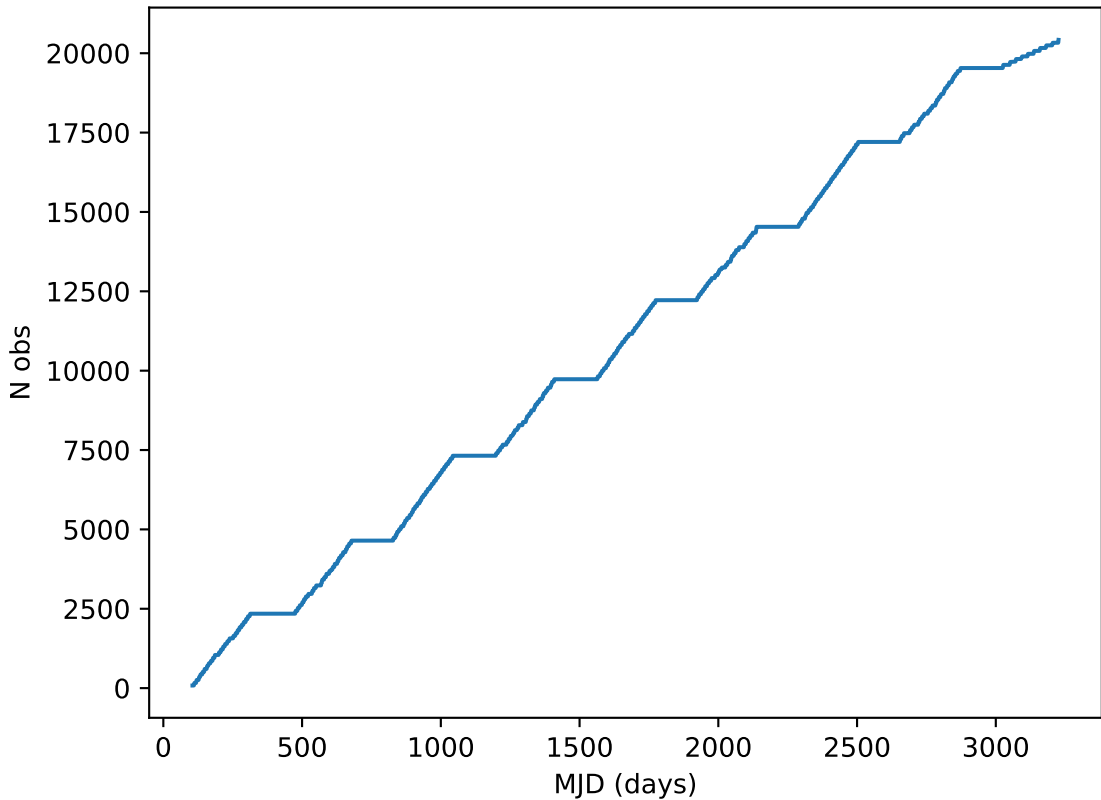
start_date_do360v3.4_10yrs all bands: DD:ECDFS Cumulative NVisits
