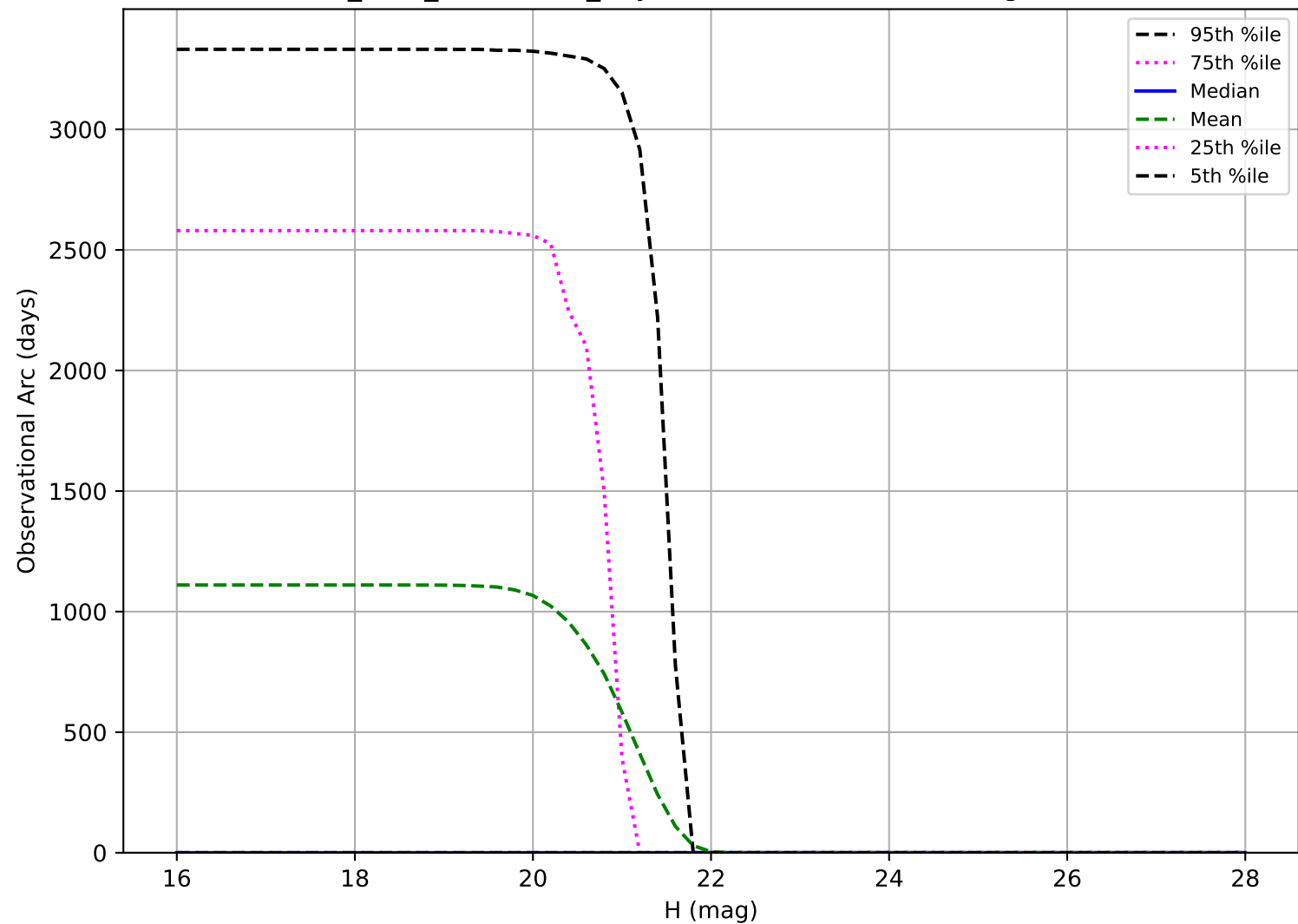
start_date_do270v3.4_10yrs: Observational Arc Length Vatira
