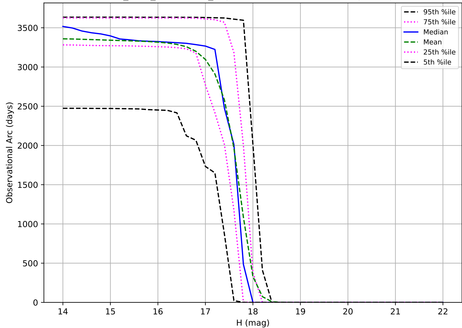
start_date_do270v3.4_10yrs: Observational Arc Length Trojan
