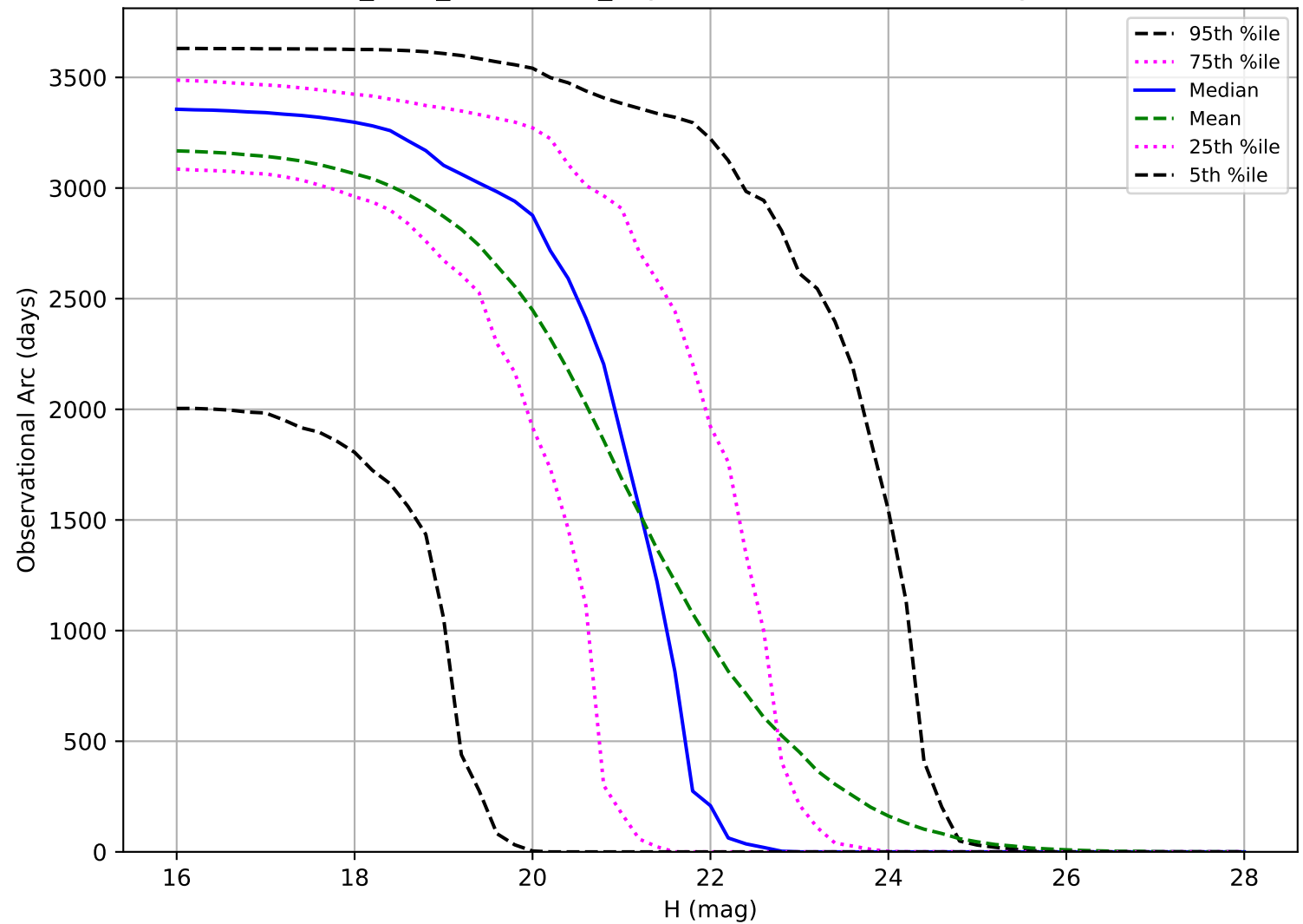
start_date_do270v3.4_10yrs: Observational Arc Length PHA
