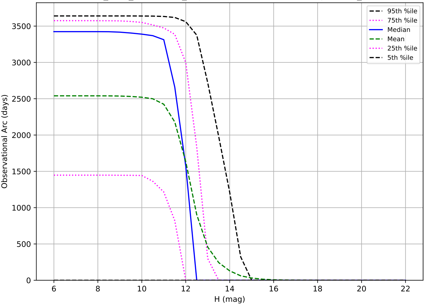
start_date_do270v3.4_10yrs: Observational Arc Length OCC_r20
