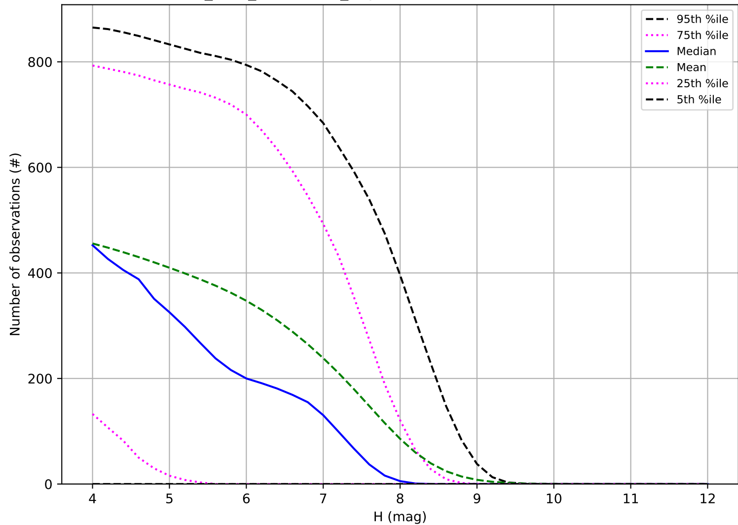
start_date_do270v3.4_10yrs: Number of observations TNO
