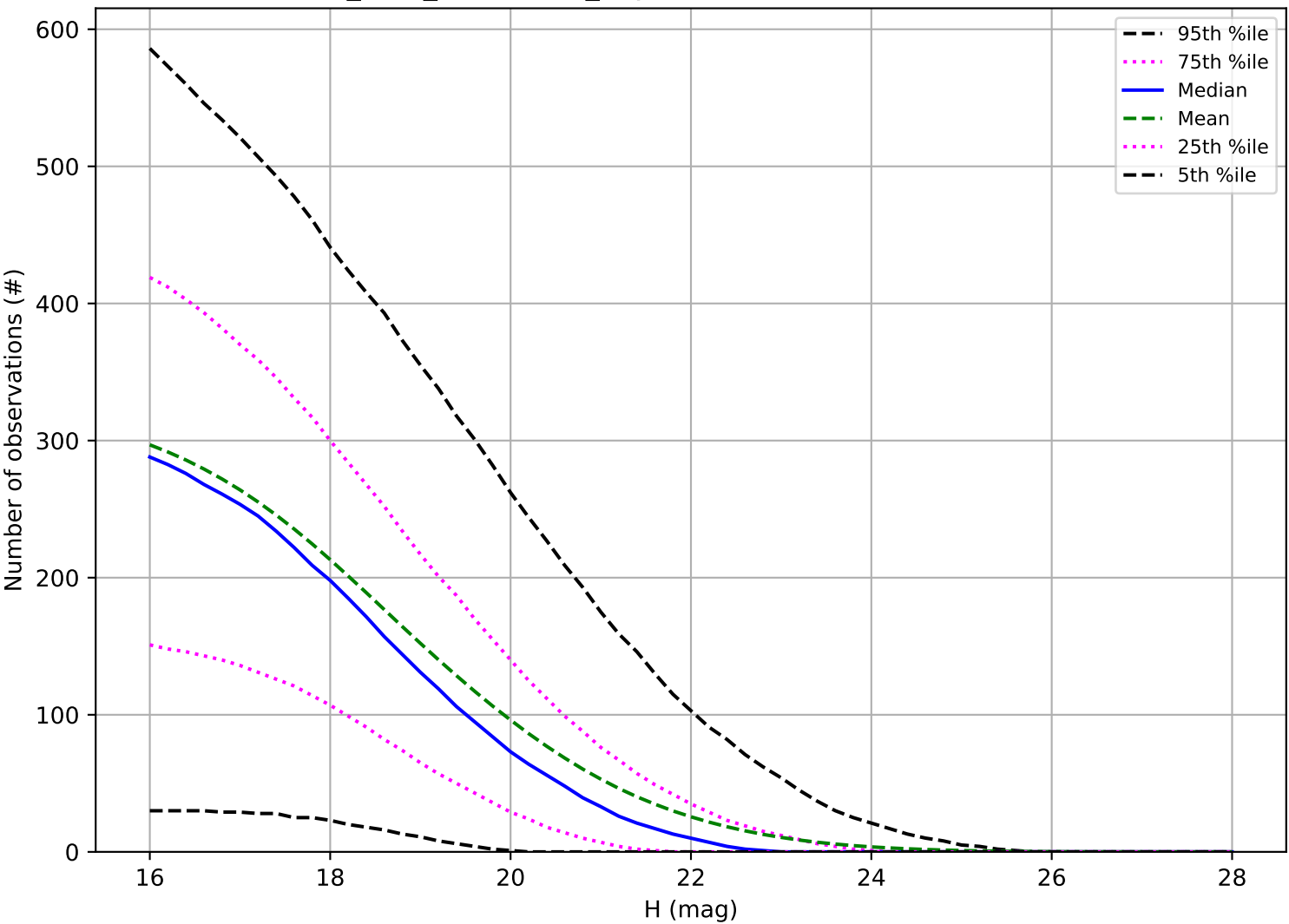
start_date_do270v3.4_10yrs: Number of observations NEO
