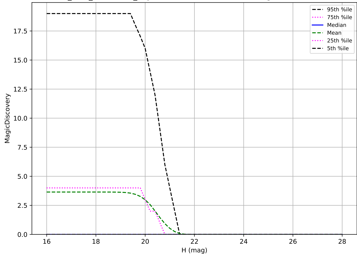
start_date_do270v3.4_10yrs: Vatira 6 detections in 60 nights detection loss
