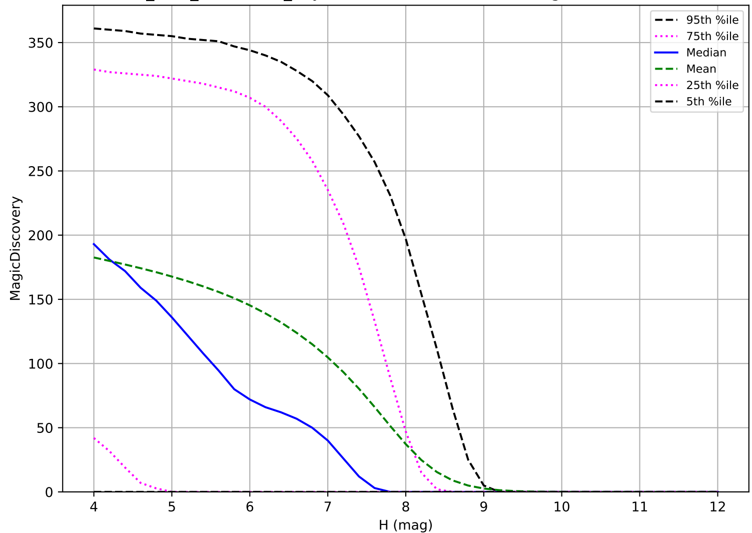
start_date_do270v3.4_10yrs: TNO 6 detections in 60 nights detection loss
