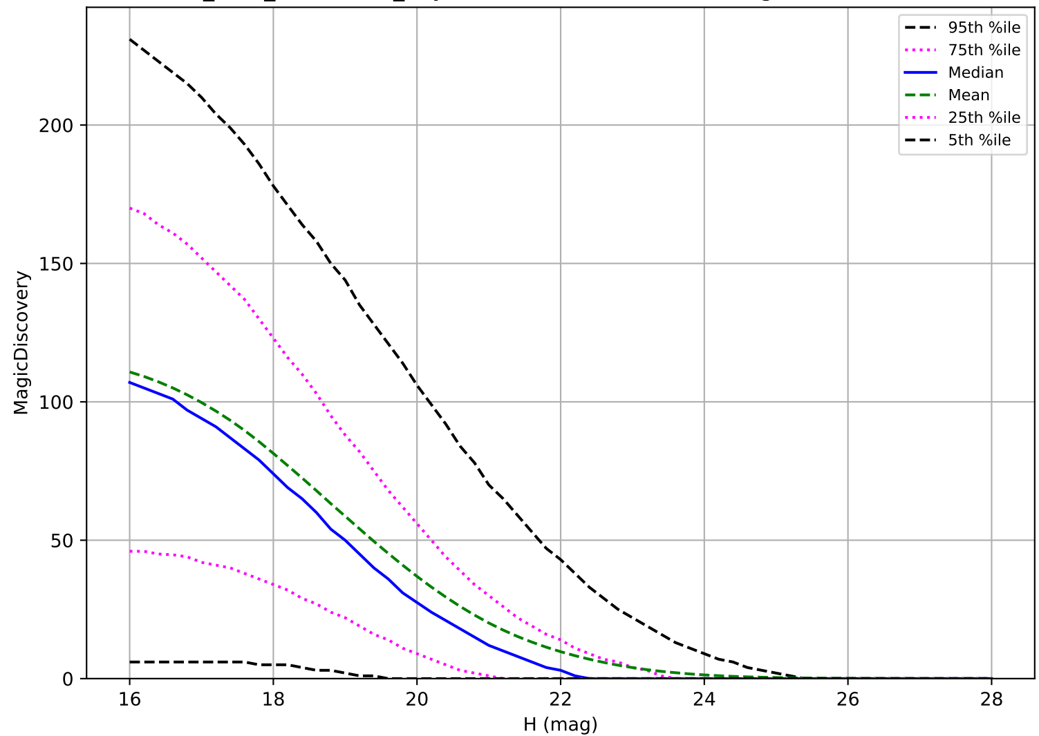
start_date_do270v3.4_10yrs: PHA 6 detections in 60 nights detection loss
