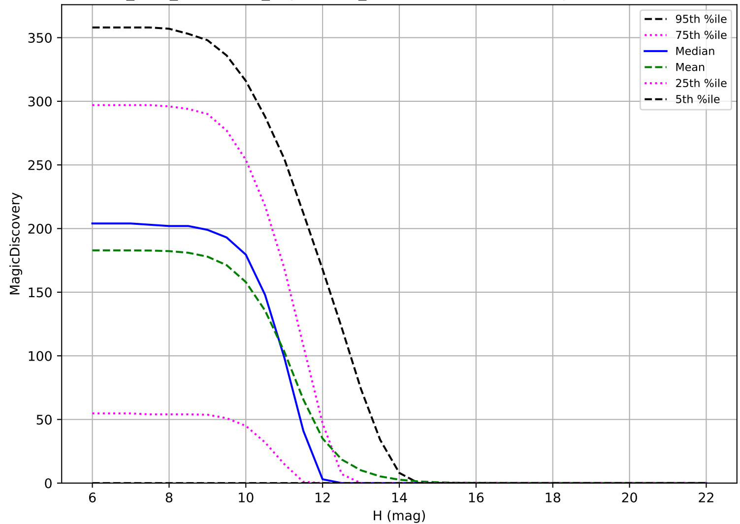
start_date_do270v3.4_10yrs: OCC_r20 6 detections in 60 nights detection loss
