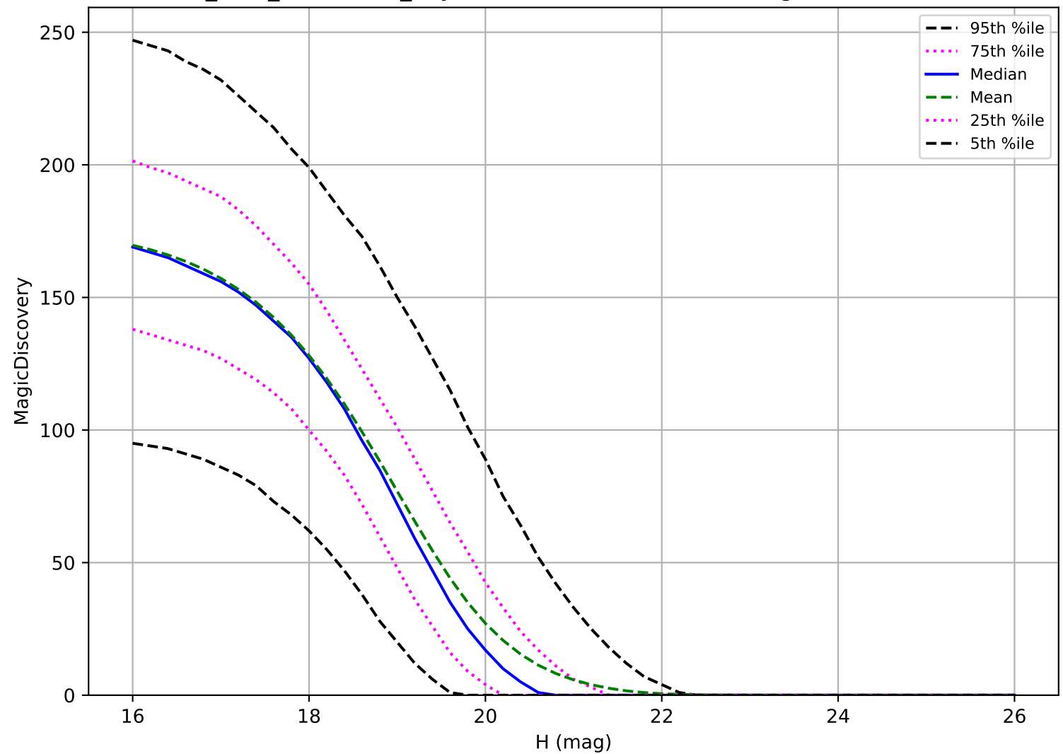
start_date_do270v3.4_10yrs: MBA 6 detections in 60 nights detection loss
