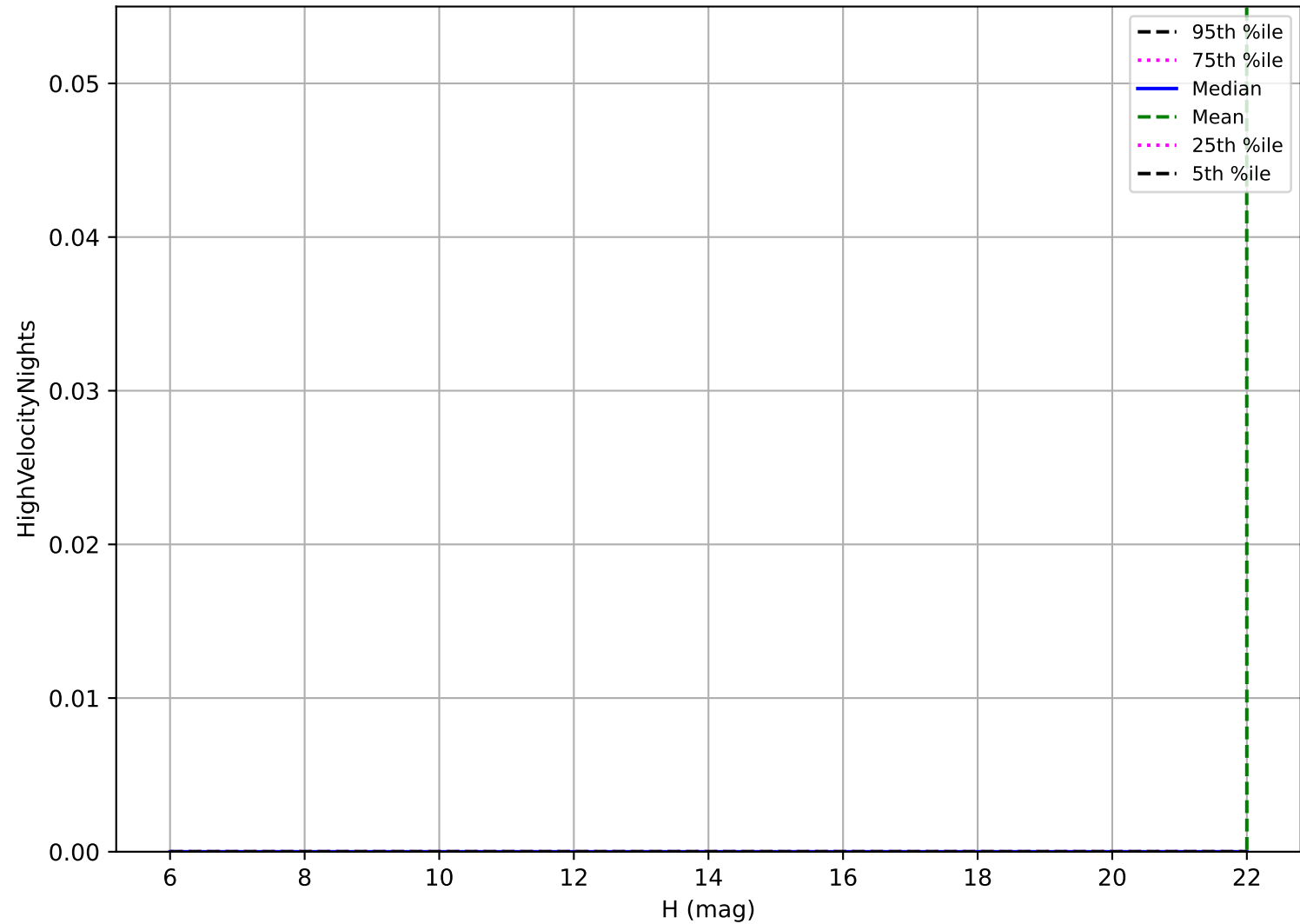
start_date_do270v3.4_10yrs: OCC_r20 High velocity pair detection loss
