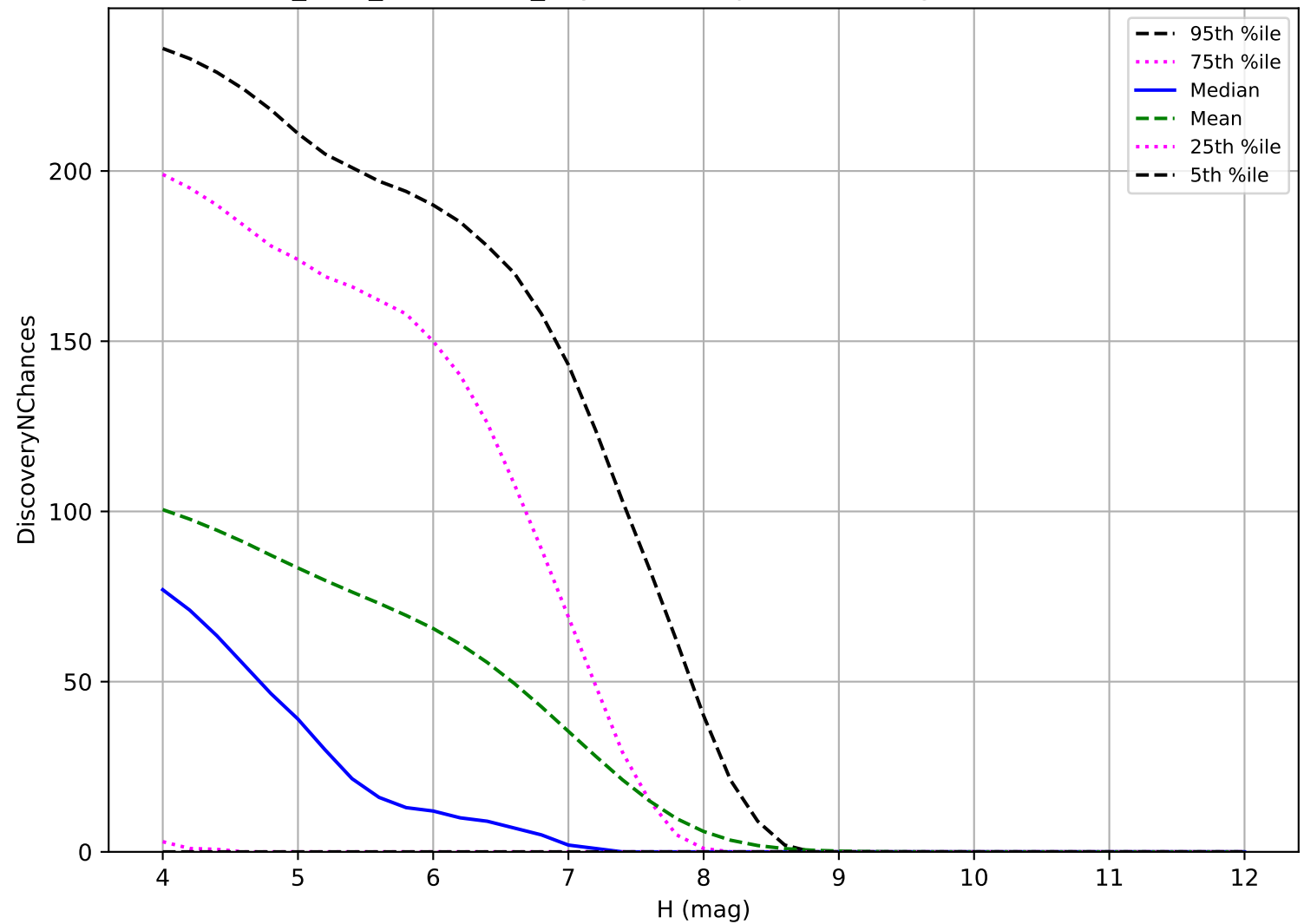
start_date_do270v3.4_10yrs: TNO 3 pairs in 15 nights detection loss
