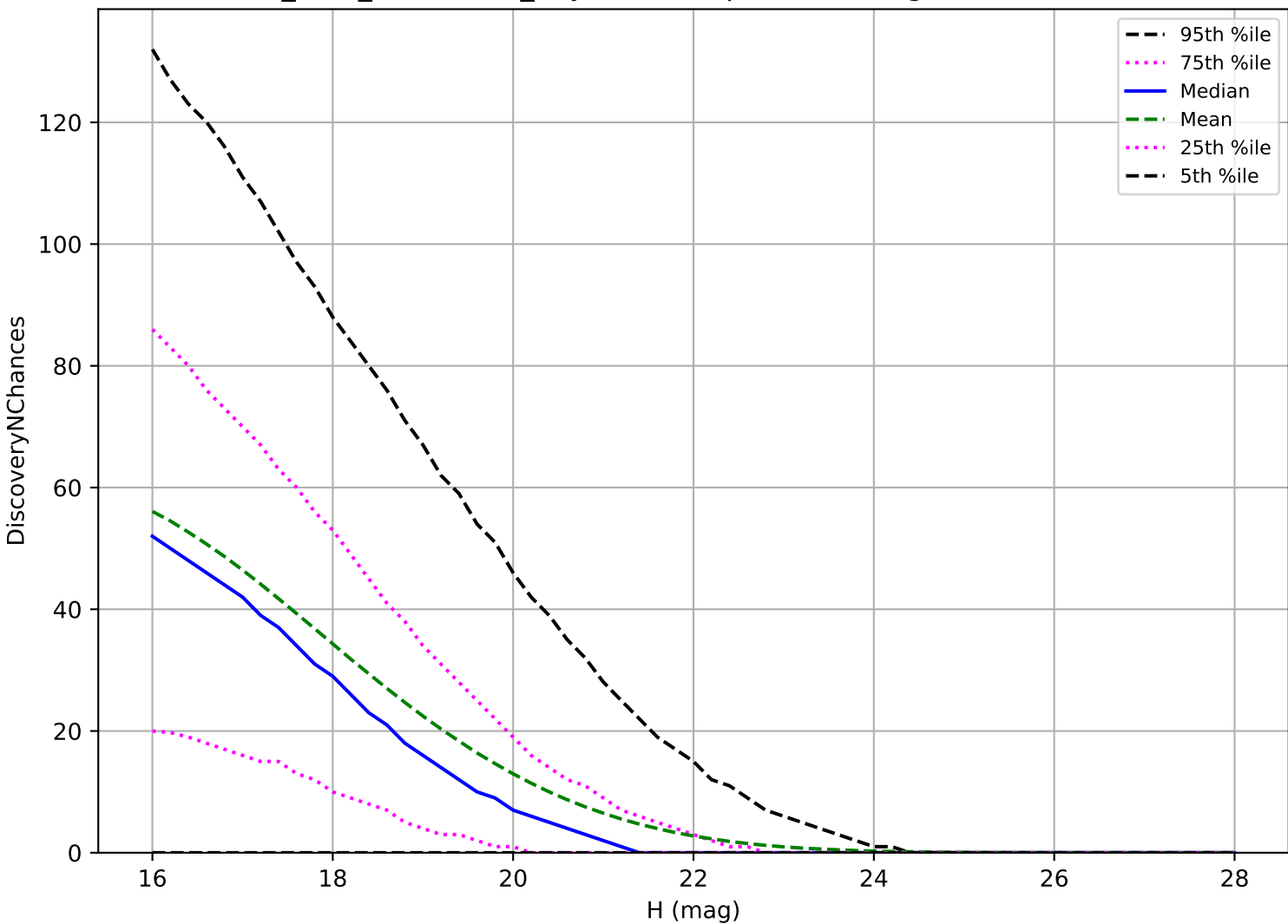
start_date_do270v3.4_10yrs: NEO 3 pairs in 15 nights detection loss
