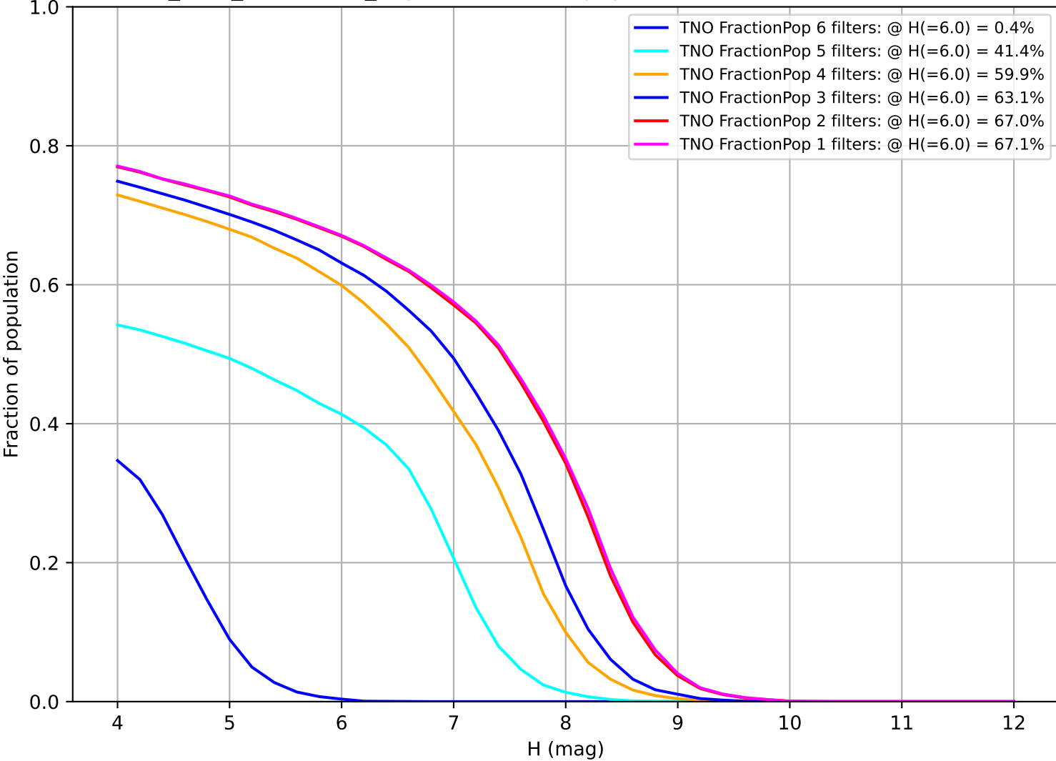
start_date_do270v3.4_10yrs: Fraction of population with colors in X filters TNO
