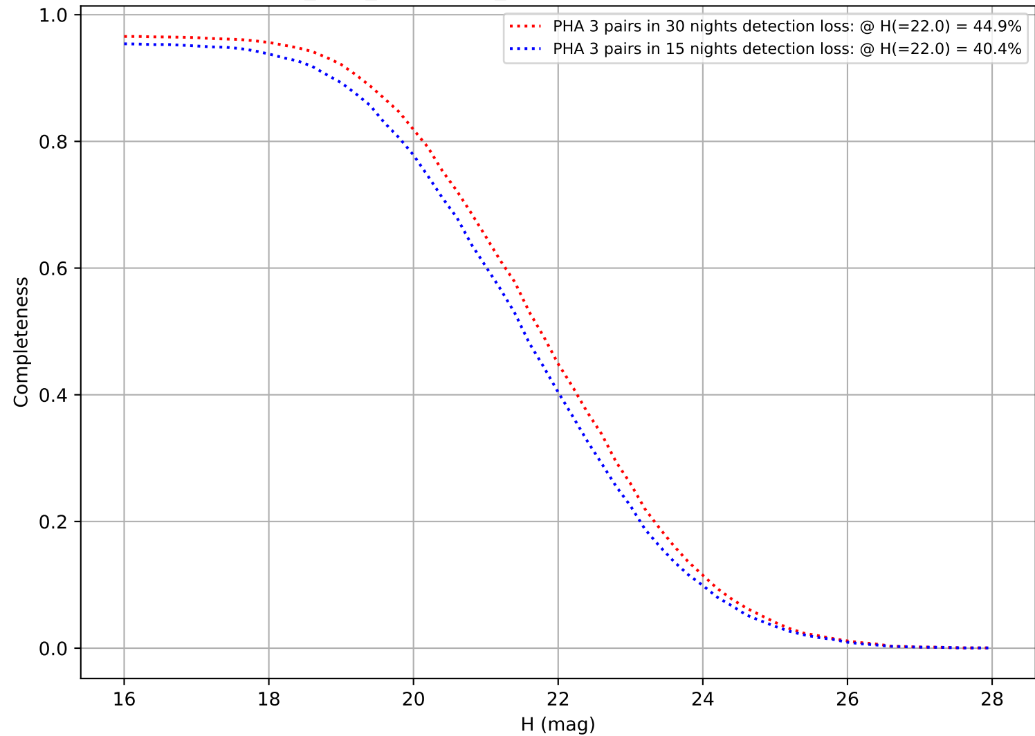
start_date_do270v3.4_10yrs: DifferentialCompleteness
