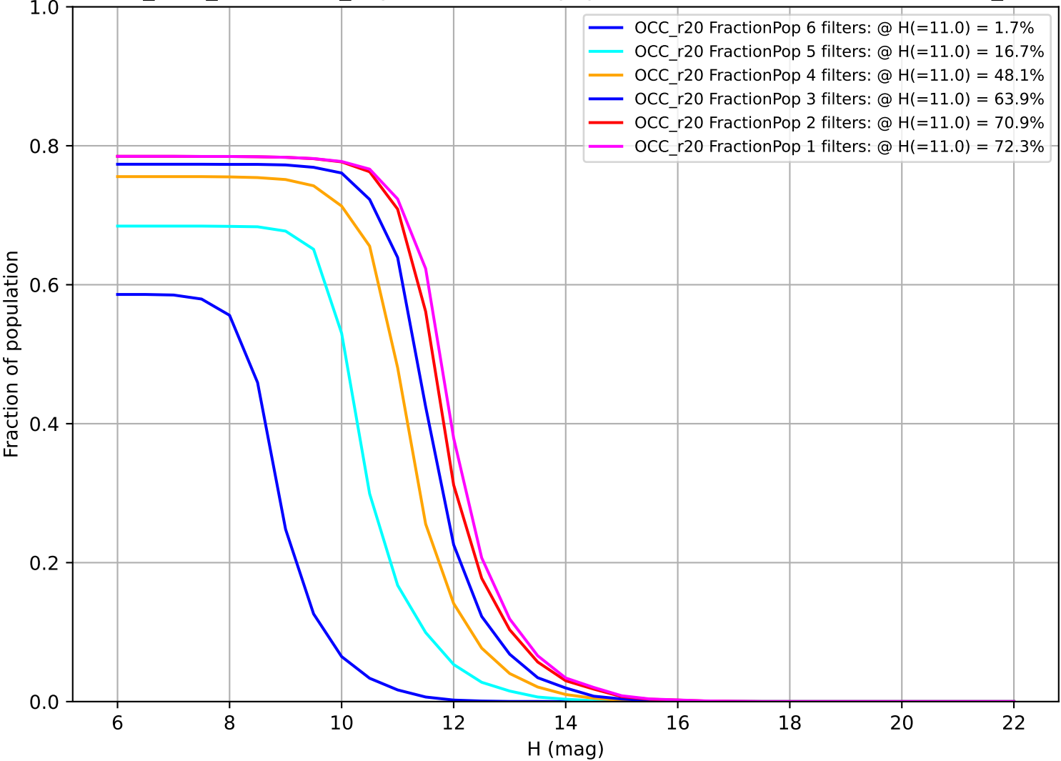
start_date_do270v3.4_10yrs: Fraction of population with colors in X filters OCC_r20
