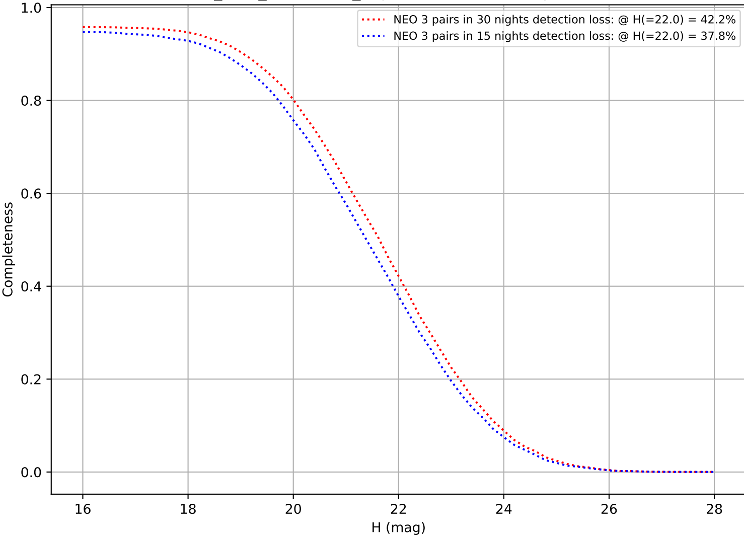
start_date_do270v3.4_10yrs: DifferentialCompleteness
