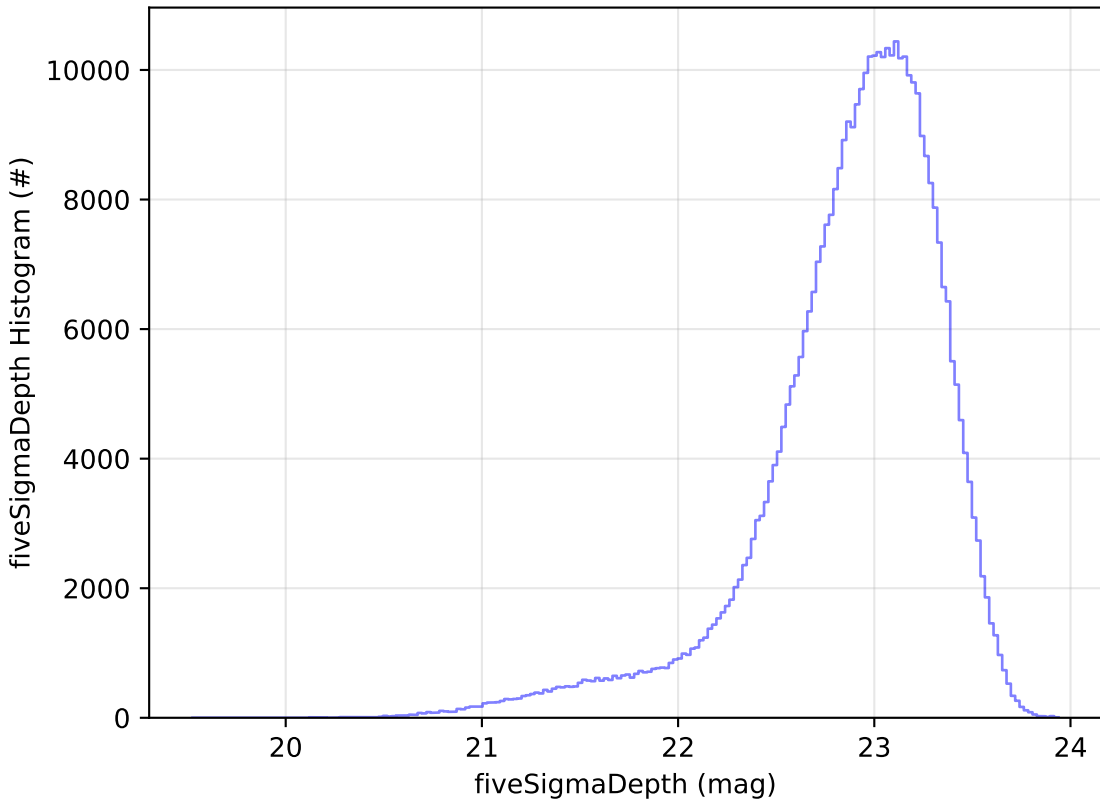
start_date_do270v3.4_10yrs z: fiveSigmaDepth Histogram
