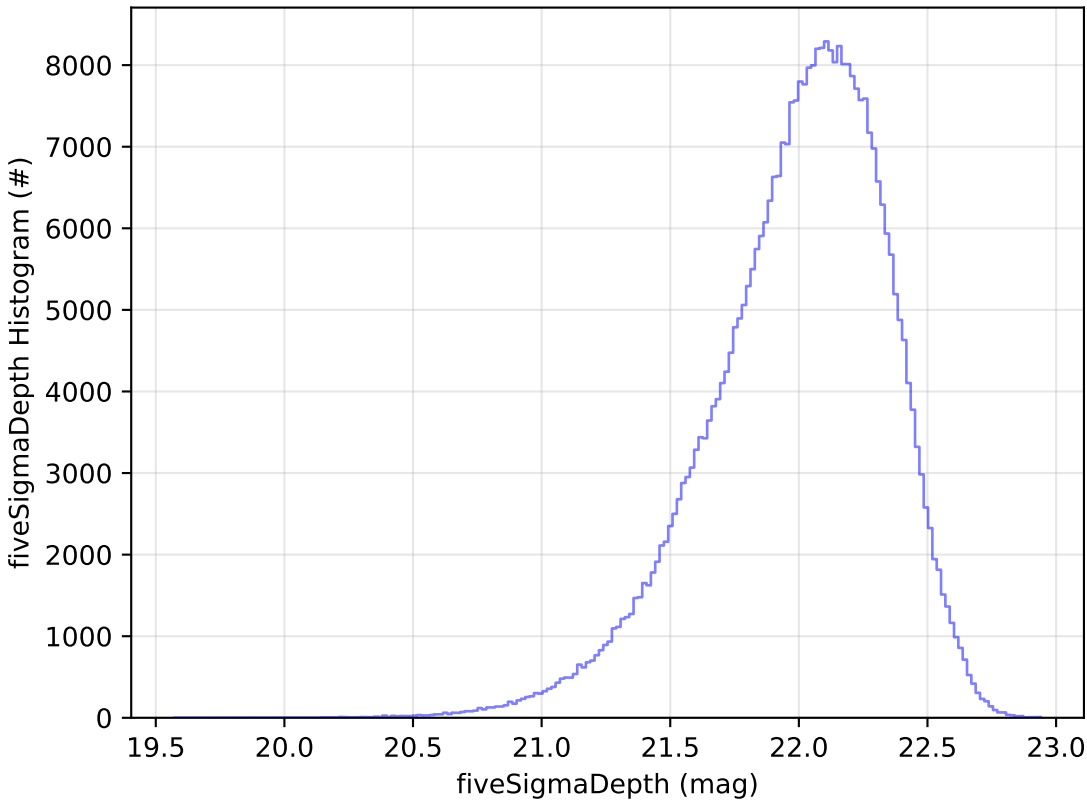
start_date_do270v3.4_10yrs y: fiveSigmaDepth Histogram
