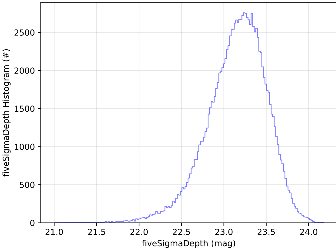
start_date_do270v3.4_10yrs u: fiveSigmaDepth Histogram
