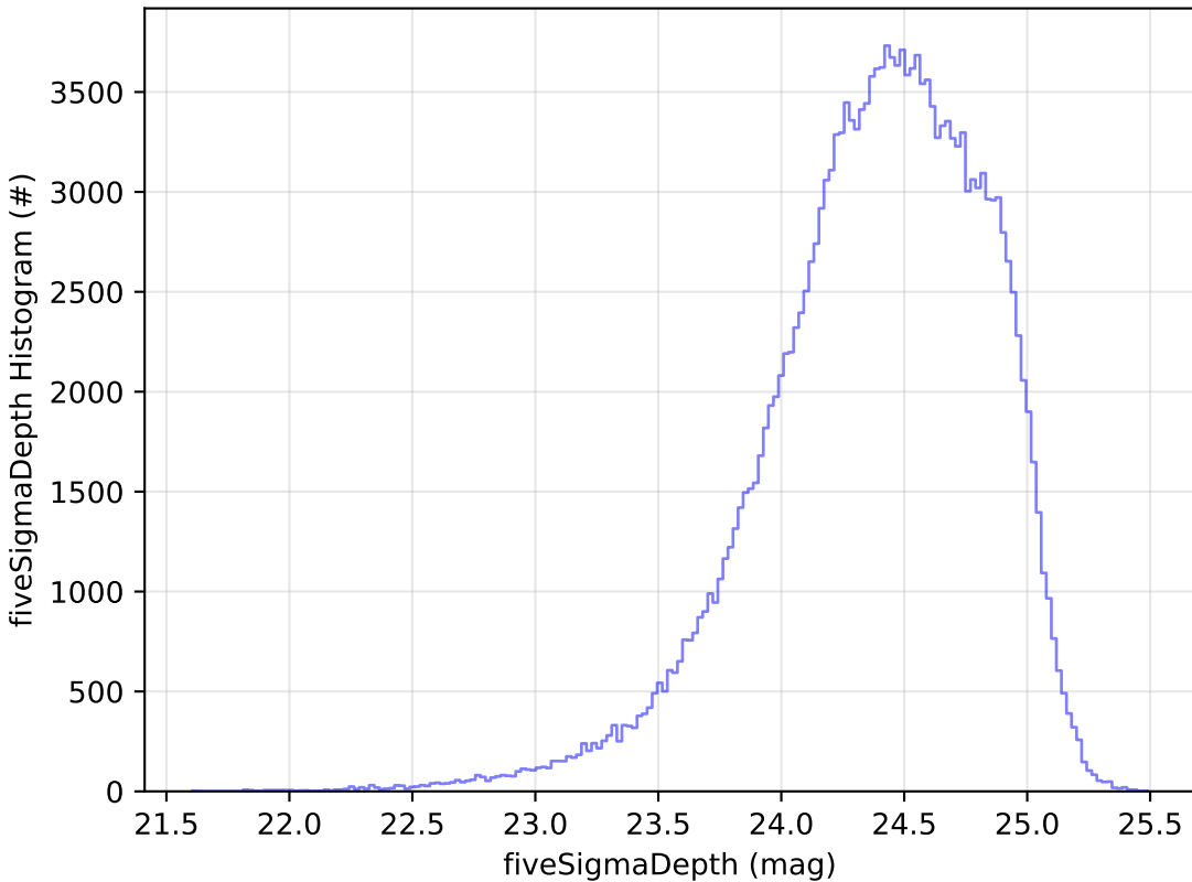
start_date_do270v3.4_10yrs g: fiveSigmaDepth Histogram
