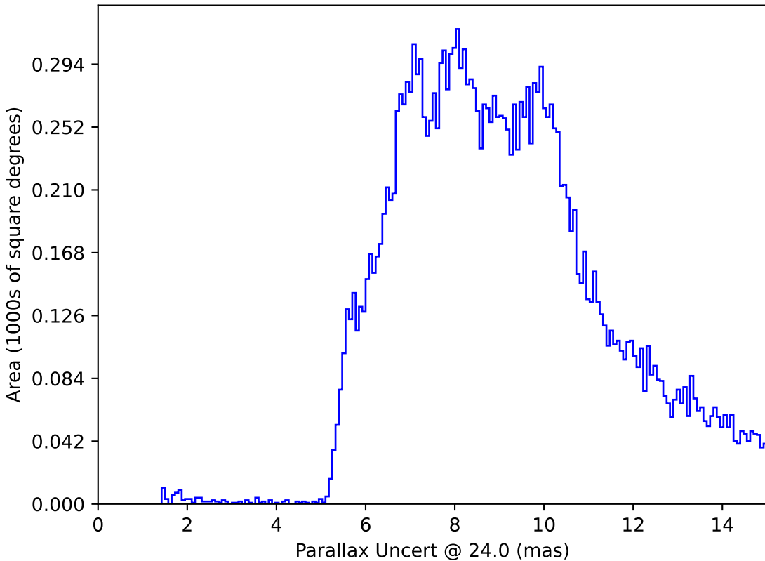
start_date_do270v3.4_10yrs : Parallax Uncert @ 24.0
