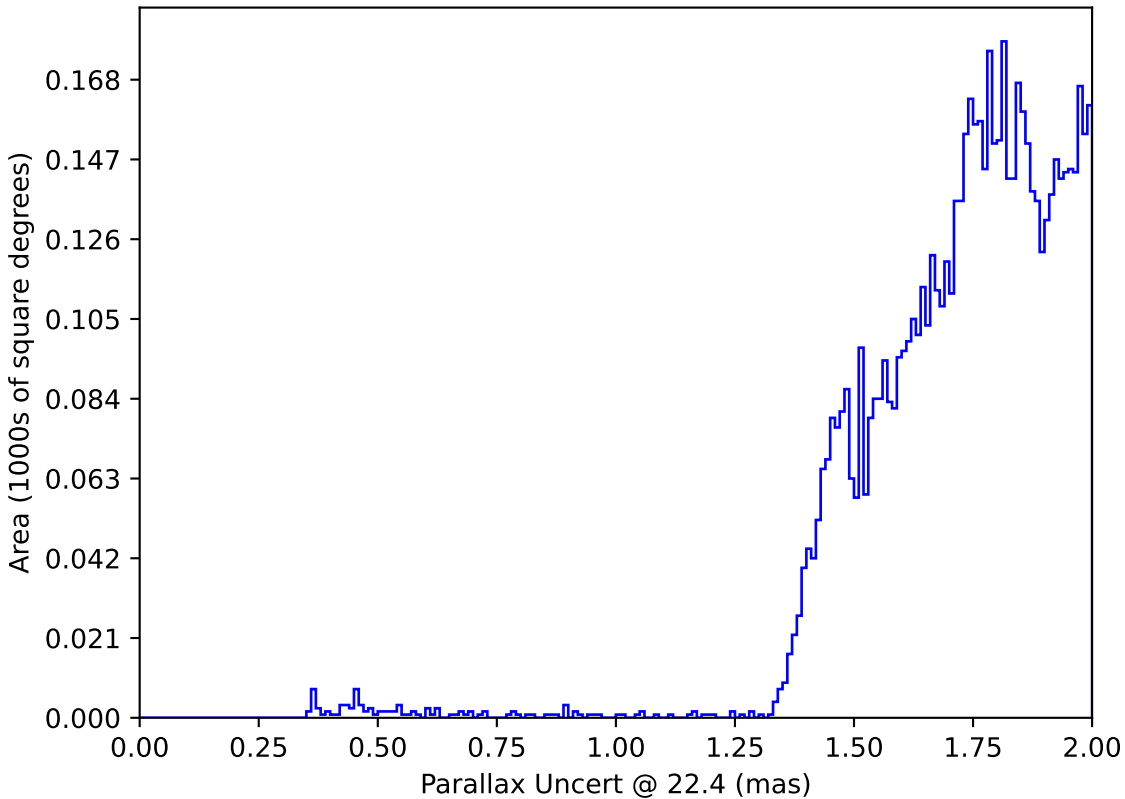
start_date_do270v3.4_10yrs : Parallax Uncert @ 22.4
